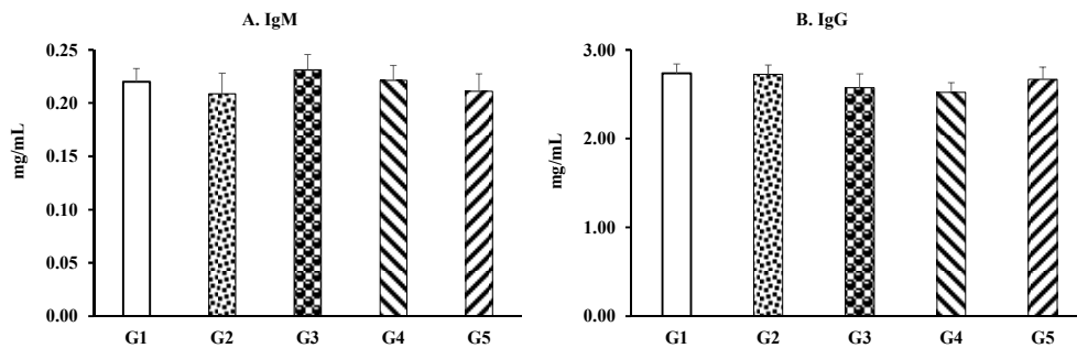
Figure 1. The effect of the test formulation on immunoglobulins (A. IgM and B. IgG) in male SD rats. G1: Normal control; G2: Disease control; G3: Levamisole; G4: Biofield Energy Treated test formulation; G5: Untreated test formulation. All the values are represented as mean \pm SEM ( n=8 ).
